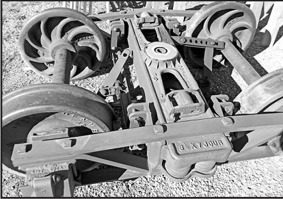
One truck with inside hung brakes and brake gear including an extra heavy brake coupling rod below the brake beam connecting the live brake lever at left and dead brake lever at right. The center plate is greased and covered with a non-historic ring of Teflon to reduce friction. – Photo © 2017 Duane Danielson.
